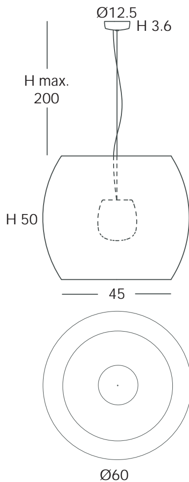
ODIP29830/60 Colgante | Suspension IP66
