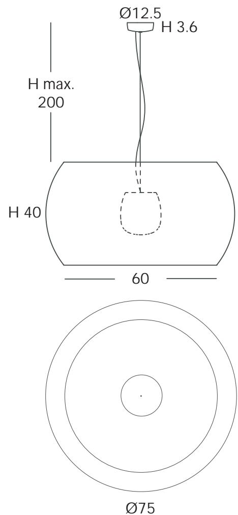
ODIP29830/75 Colgante | Suspension IP66
