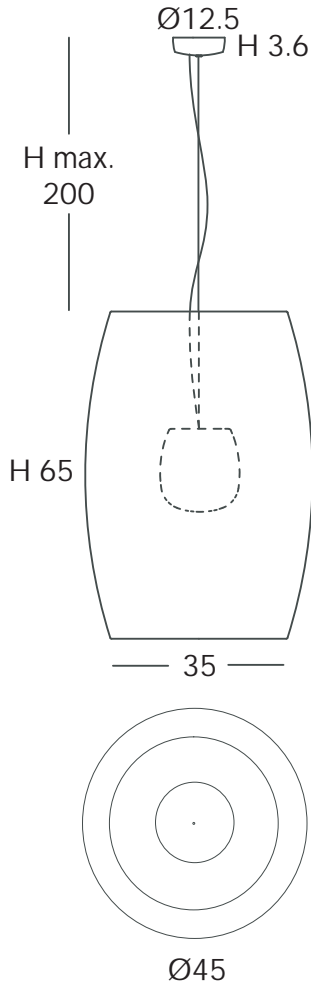
ODIP29830/45 Colgante | Suspension IP66
